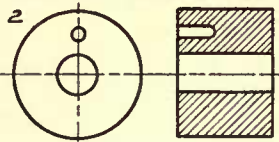
SIDE VIEW IN SECTION.
